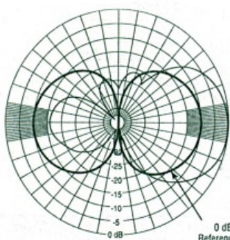
VERTICAL PATTERN
